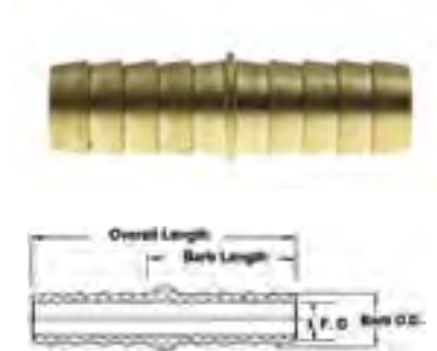
Barb x Barb Fitting allowing for Joining Hoses
