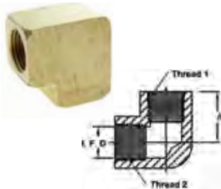
Female x Female Elbow
