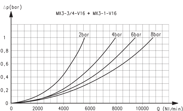
Diagram for electro-pneumatic control valves MX3
