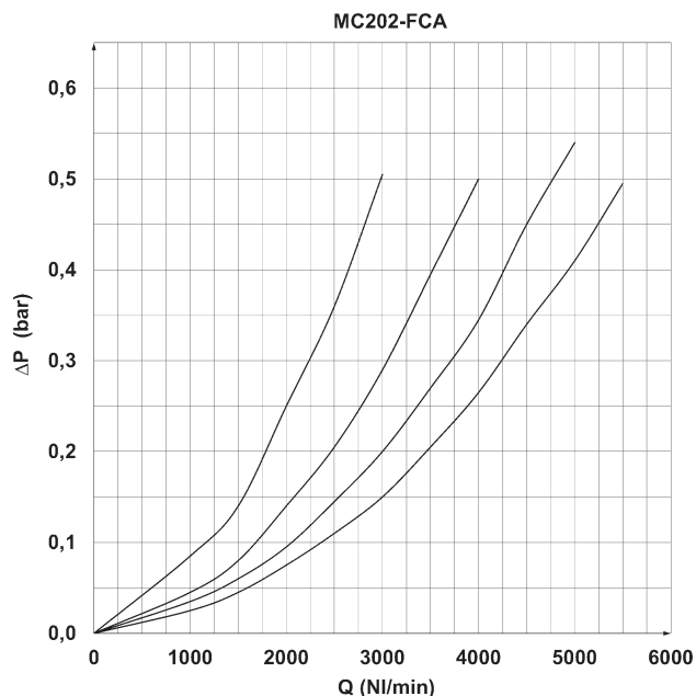
Flow diagram for model: MC202-FCA
