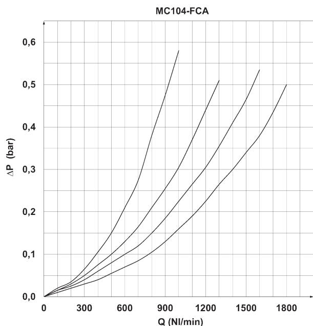
Flow diagram for model: MC104-FCA
