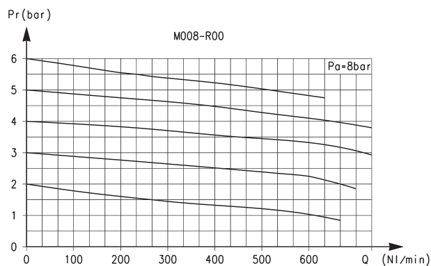
Flow diagram for models: M008-R00
