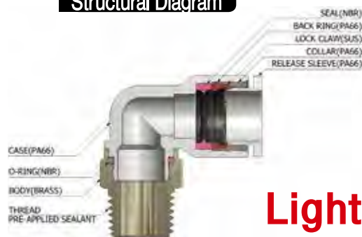
Structural Diagram
