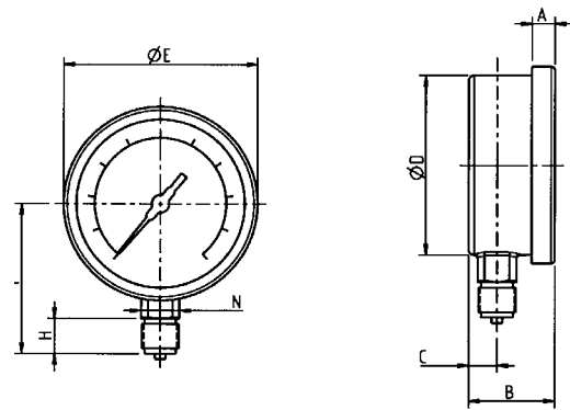
Bottom connection.
