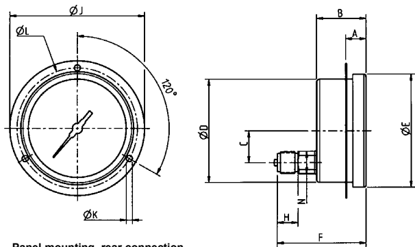
Panel mounting, rear connection.
