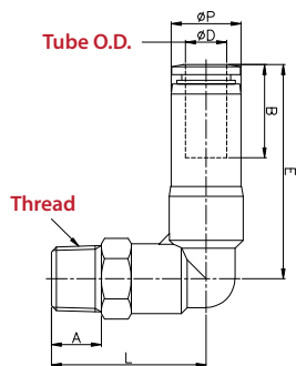
Metric Tube BSPP(G) Thread
