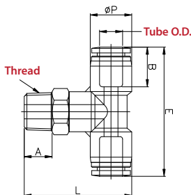
Metric Tube BSPP(G) Thread
