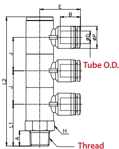
Metric Tube BSPP(G) Thread
