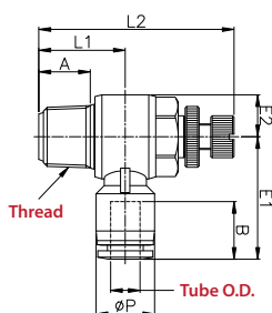
Metric Tube BSPP(G) Thread
