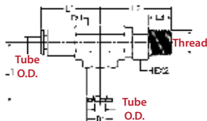
Inch Tube NPT Thread Metric Tube BSPT(R) Thread
