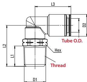
Inch Tube NPT Thread Metric Tube BSPT(R)
