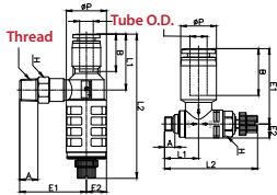
Metric Tube BSPT(R) Thread
