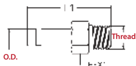
Inch Tube NPT Thread Metric Tube BSPT(R) Thread
