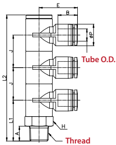
Metric Tube BSPP(G) Thread
