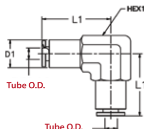
Inch Tube & Metric Tube
