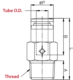
Inch Tube NPT Thread
