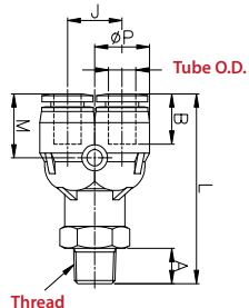
Metric Tube BSPT(R) Thread
